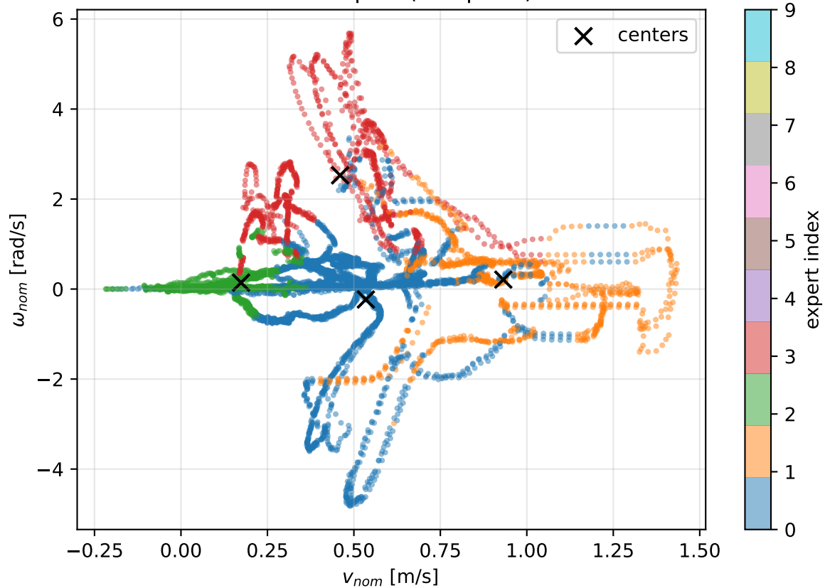
Active expert (4 experts)
