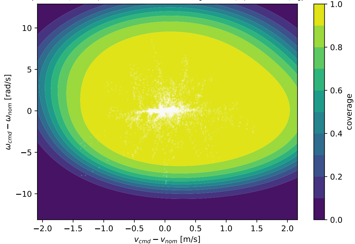
Residual coverage vs command offset (0 = off / OOD; state fixed at mean [0.44 m/s, 0.23 rad/s])
